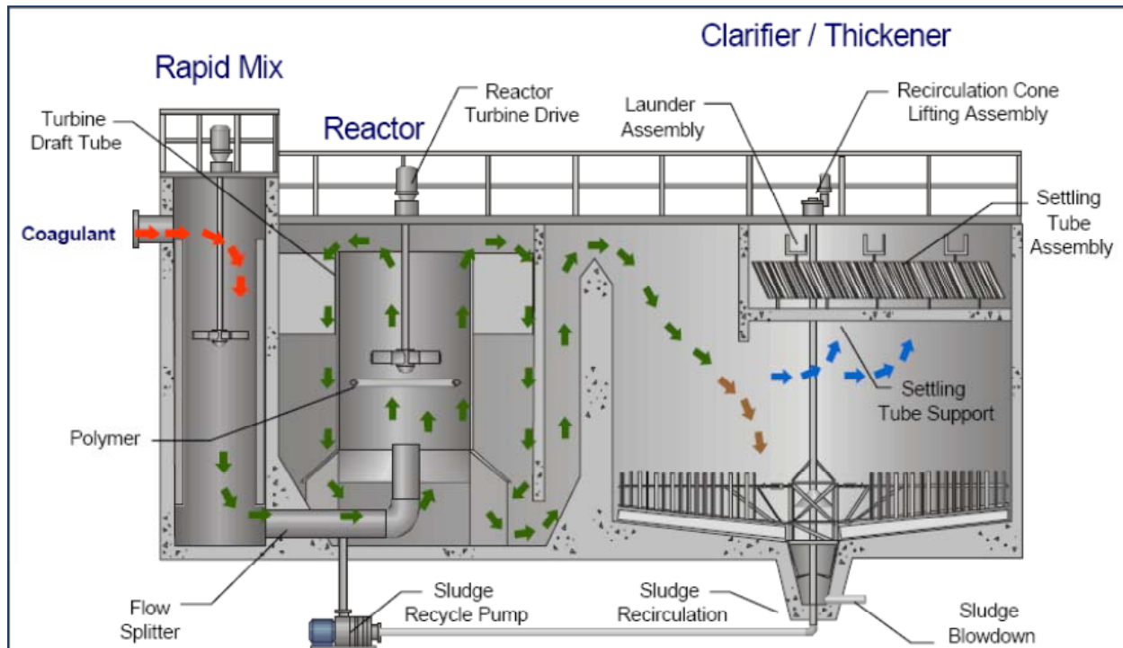
Figure 9: High-Rate Clarification
