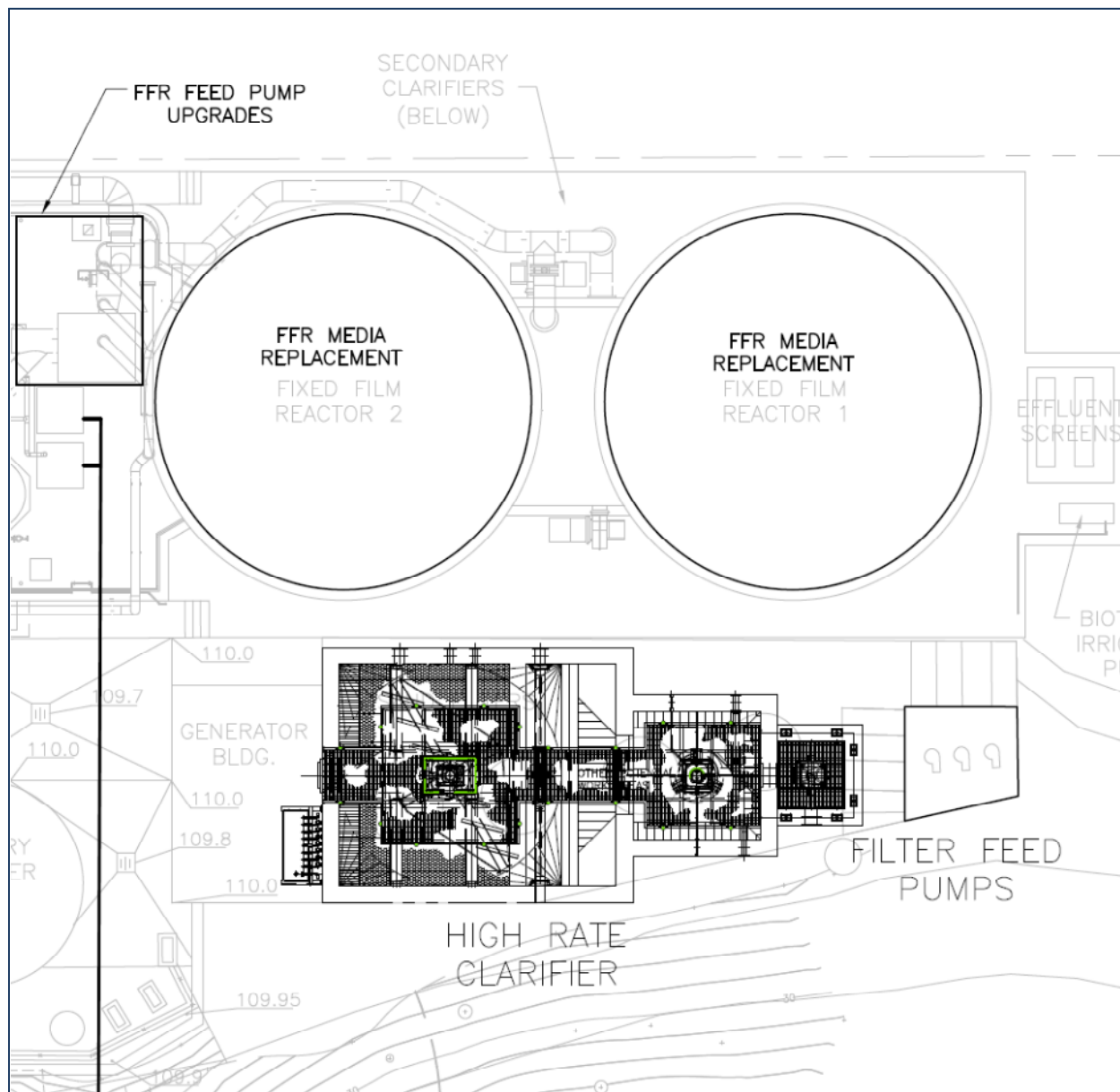
Figure 10: Preliminary 4.5 MGD High Rate Clarifier Layout
