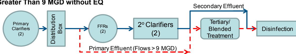
Figure 4: Flow Path at Greater Than 9 MGD (without Equalization)
