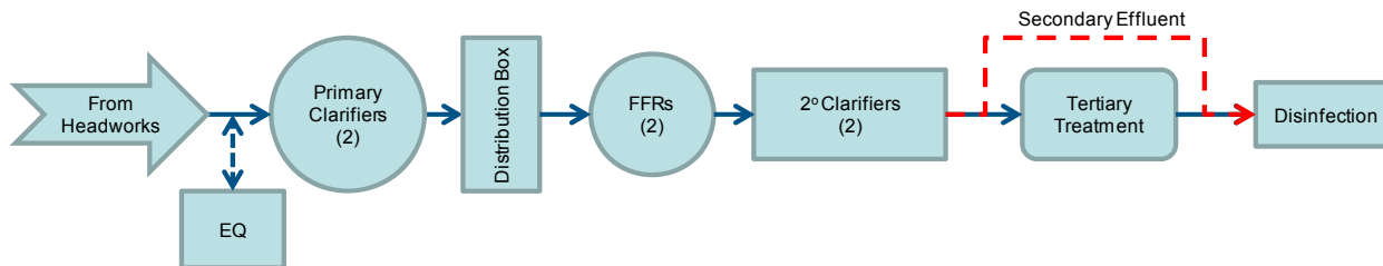
Figure 5: Flow Path with Equalization
