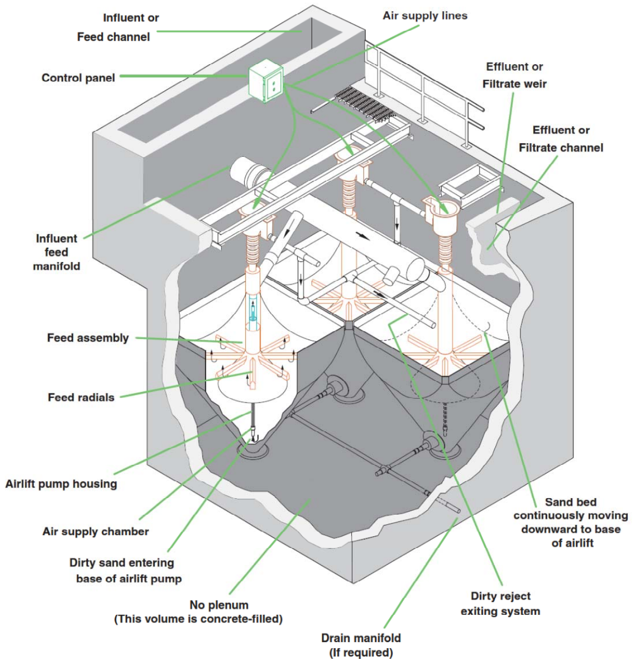
Figure 7: Upflow Continuous Backwash Filter Installed in Concrete Tanks (Parkson Dynasand)
