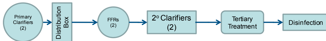
Figure 3: Normal Flow Treatment Flow Path for Flows Up to 6 MGD and 9 MGD
