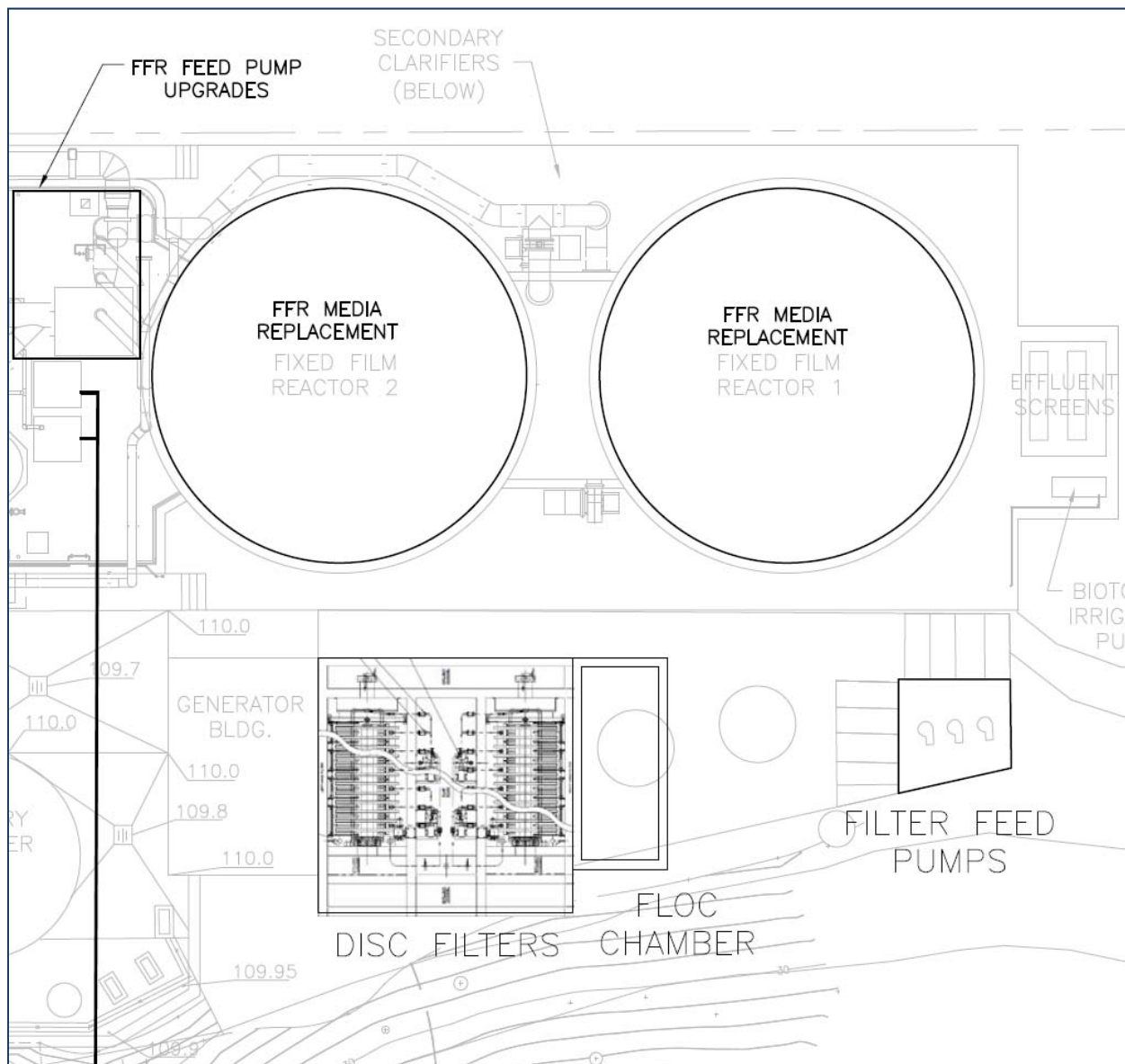
Figure 12: Preliminary 6.0 MGD Disk Filter Layout
