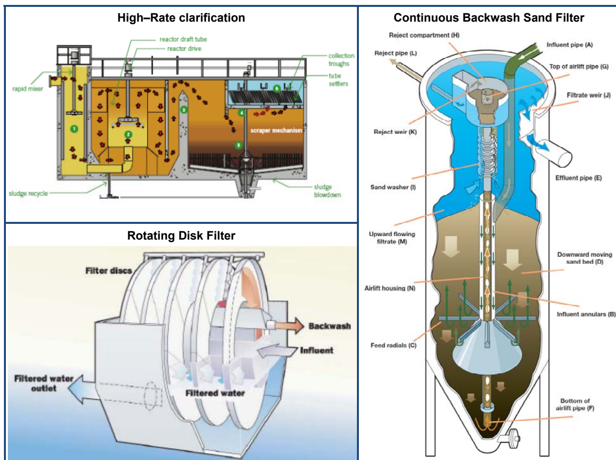
Figure 6: Potential Tertiary Treatment Technologies
