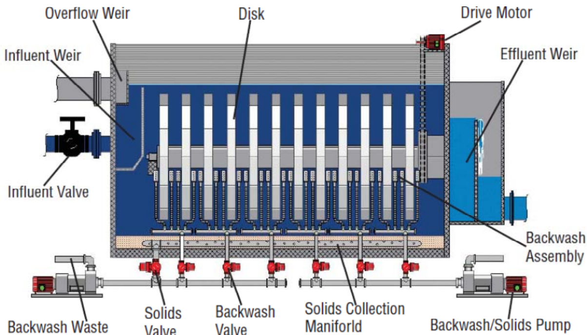
Figure 11: Rotating Disk Filter
