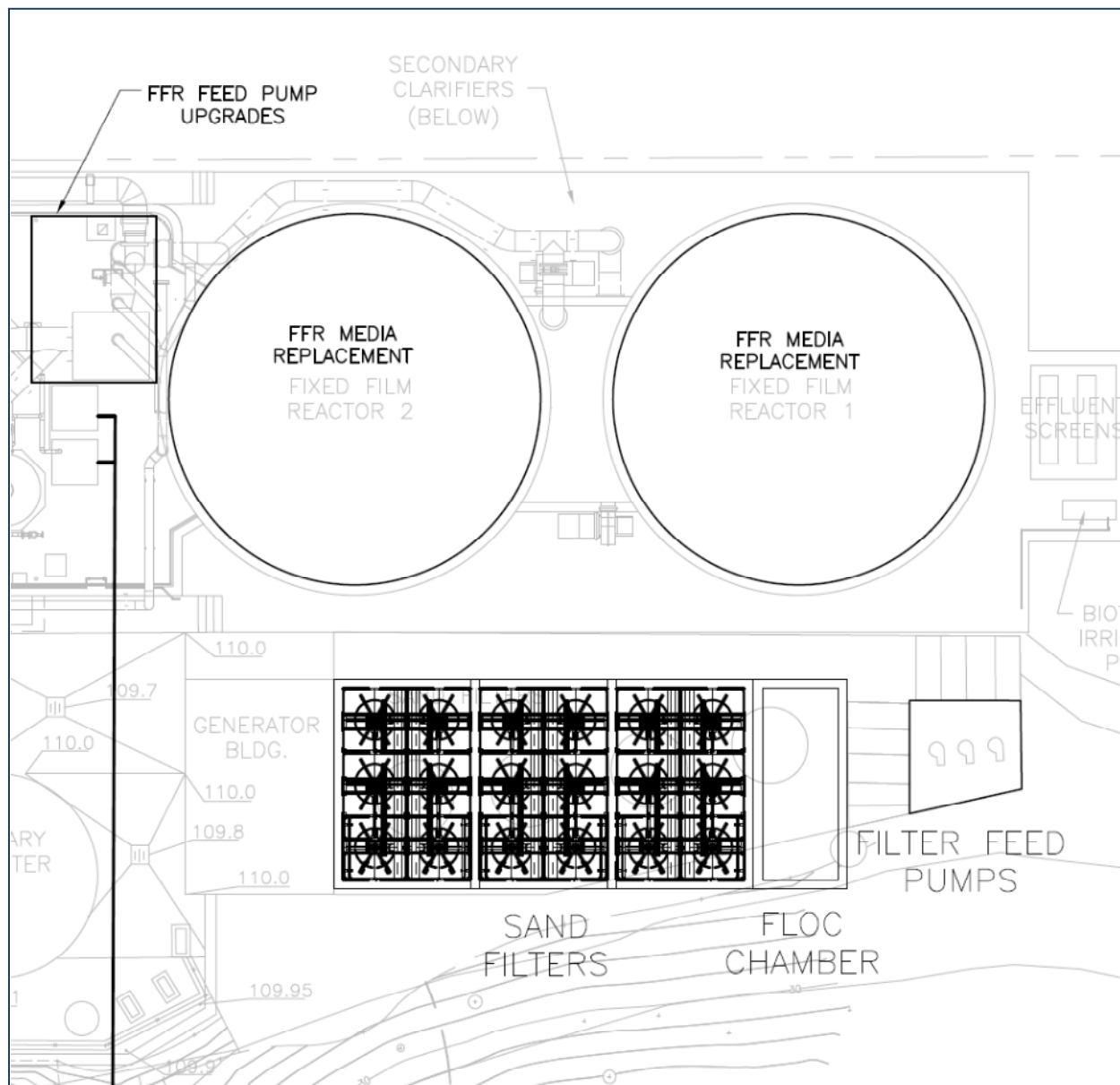
Figure 8: Preliminary 5.0 MGD Sand Filter (Upflow Continuous Backwash Type) Layout
