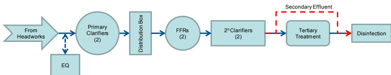
Figure 13: Flow Path with Equalization
